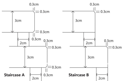
Anti-Slipping Type 2
